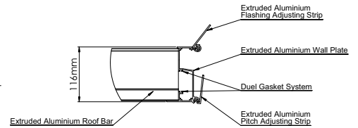
Wall Plate & Roof Bar Section
