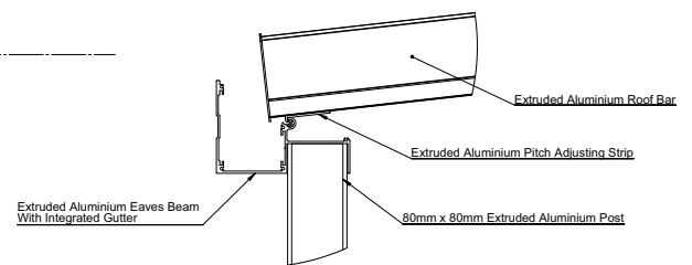
Eaves Beam Roof Bar & Post Section
